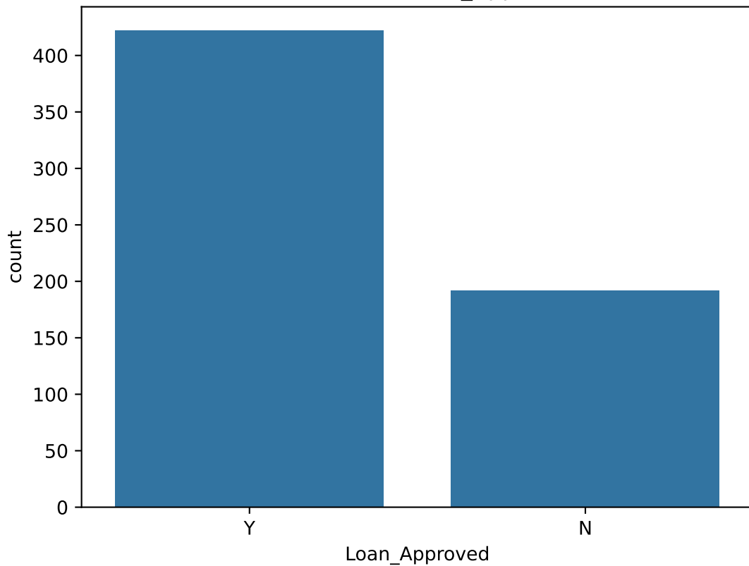
Count Plot of Loan_Approved
